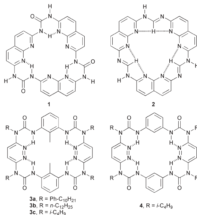
Fig. 1 Macrocycles 1–4 synthesized in one step utilizing the propensity to form intramolecular H-bonding to guide the ring closing reaction.
