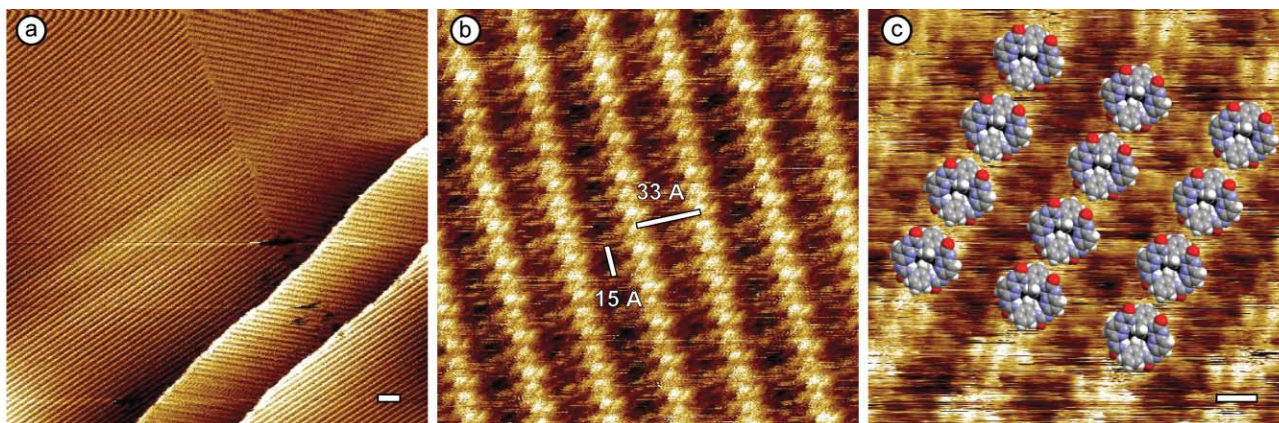
Fig. 3 STM image of 3b self-assembly on HOPG from 1,2,4-trichlorobenzene in constant current mode using a Pt/Ir tip. (a) Large scan area with step edges and grain boundaries: I_{\text{set}} = 26.9 pA, V_{\text{set}} = -564 mV, scale bar is 10 nm. (b) Lamellar structure with periodicities of 33 Å (lamellae) and 15 Å (substructure in each lamella), respectively: I_{\text{set}} = 95.5 pA, V_{\text{set}} = -1.00 V. (c) A CPK model of 3b superimposed onto the STM image, alkyl chains are omitted for clarity, same conditions as (b), scale bar is 1 nm.
