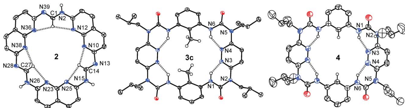
Fig. 2 ORTEP crystal structure views of macrocycles 2 , 3c and 4 . Thermal ellipsoids are shown at the 50% probability level and solvents and selected hydrogen atoms were removed for clarity.
